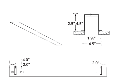
RECESSED TRIMLESS RT - Recessed Trimless Bracket PO - Power Opening *Cutout Dimensions = Total Length x Width of Extrusion.
