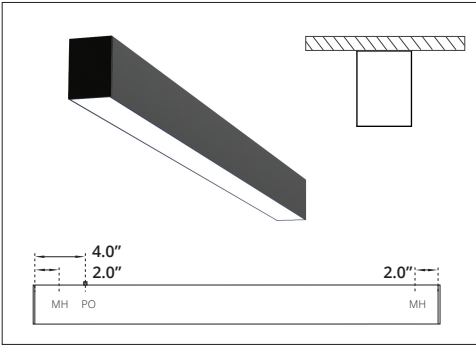
SURFACE MOUNT MH - Mounting Hole PO - Power Opening
