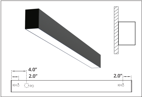
WALL FLUSH KH - Key Hole PO - Power Opening
