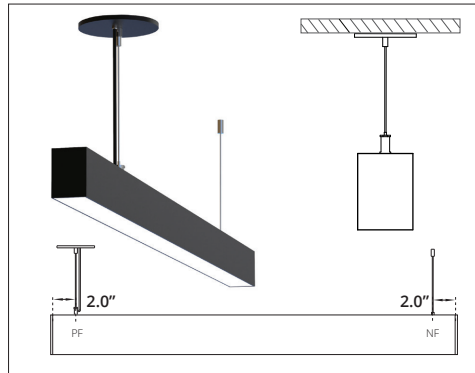
SUSPENDED
