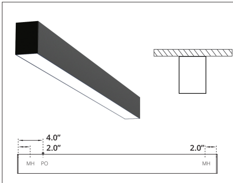
SURFACE MOUNT
