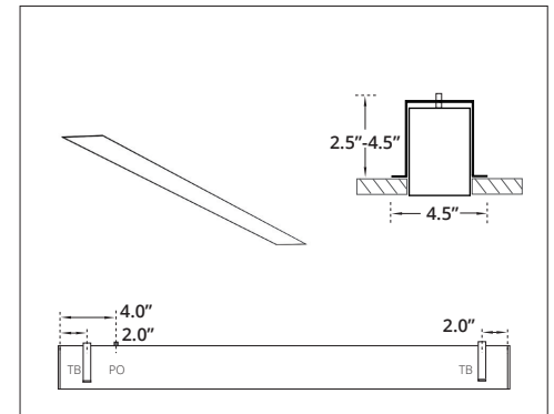
RECESSED TRIMLESS
