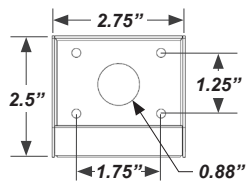
Bracket Dimensions
