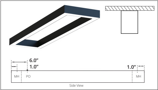
SURFACE MOUNT MH - Mounting Hole PO - Power Opening
