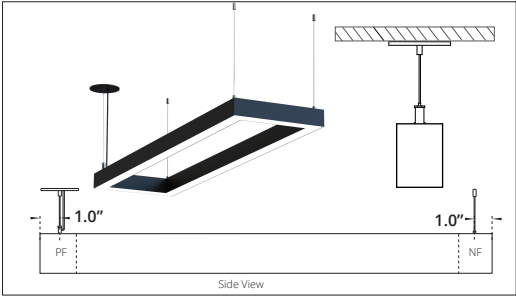
SUSPENDED PF - Power Feed NF - Non Power Feed
