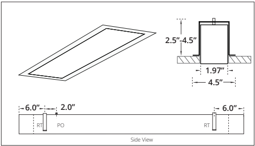
RECESSED TRIMLESS RT - Recessed Trimless Bracket PO - Power Opening *Cutout Dimensions = Total Length x Width of Extrusion.
