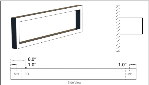
WALL FLUSH MH - Mounting Hole PO - Power Opening
